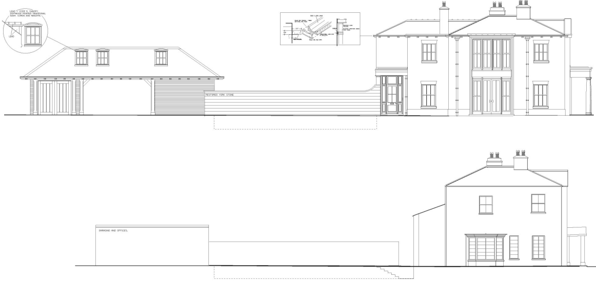
AS EXISTING SIDE ELEVATION - West.
